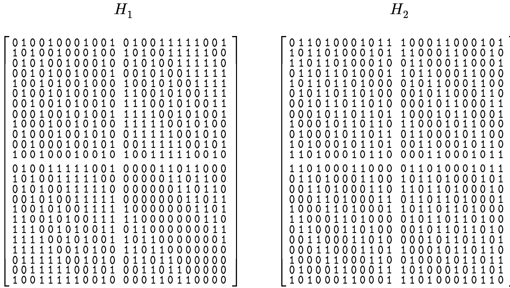
Figure 1. Adjacency matrices for H_1 and H_2 .
