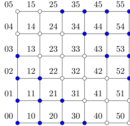
Figure 2: An FPDS and SPDS S in blue
