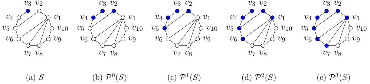
Figure 5: A graph G with \bar{\gamma}_p(G) = 0 as in Theorem 4.6, item 4. S = \{v_3\} is shown in blue on the left, followed by \mathcal{P}^0(S) through \mathcal{P}^3(S) . Continuing, \mathcal{P}^4(S) = \{v_1, v_2, \dots, v_8\} , and \mathcal{P}^5(S) = V .
