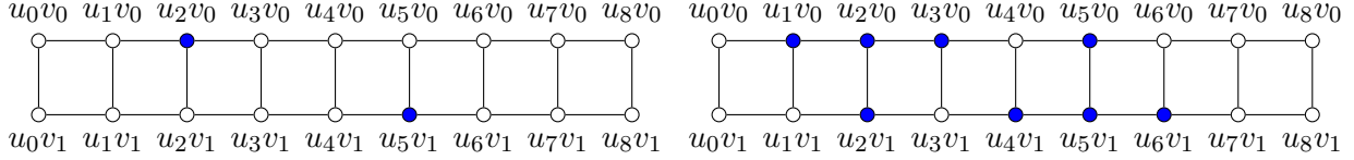
Figure 6: A ladder graph, P_9 \square P_2 with FPDS S in blue on the left and \mathcal{P}^0(S) in blue on the right.
