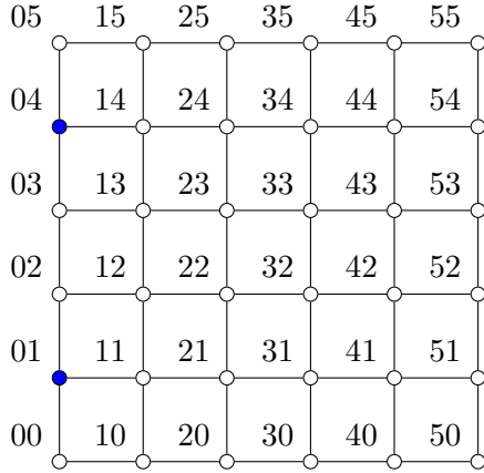
Figure 1: A PDS S in blue
