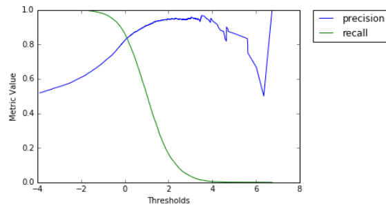
(b) Classifier performance )
