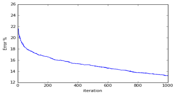
(a) classifier learning curve
