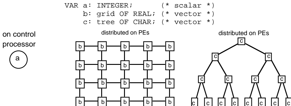
Figure 1.5: Allocation of scalar and vector data
