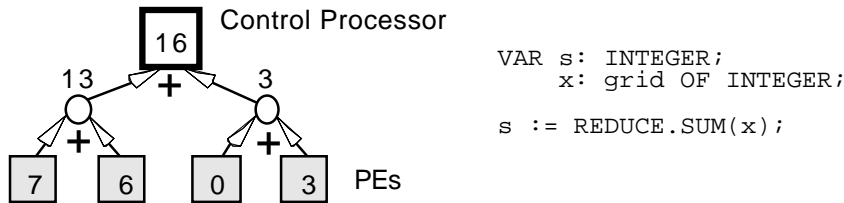
Figure 1.12: Vector reduction in Parallaxis
