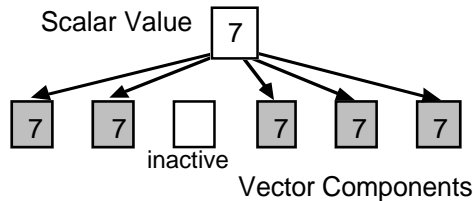
Figure 1.11: Data exchanges between PEs and control processor
