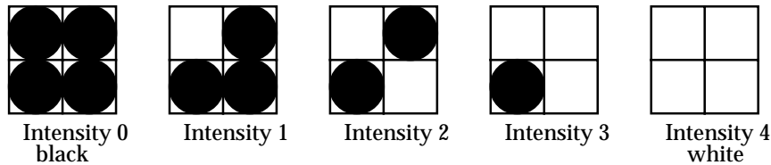
Figure 2.8: Dithering with 2 \times 2 pattern
