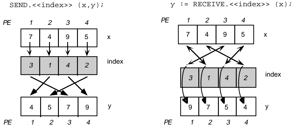
Figure 1.10: Unstructured data exchange
