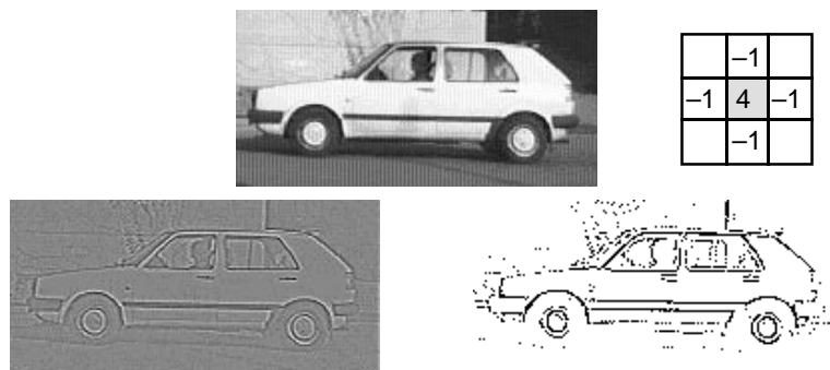
Figure 2.7: Edge detection with Laplace operator
