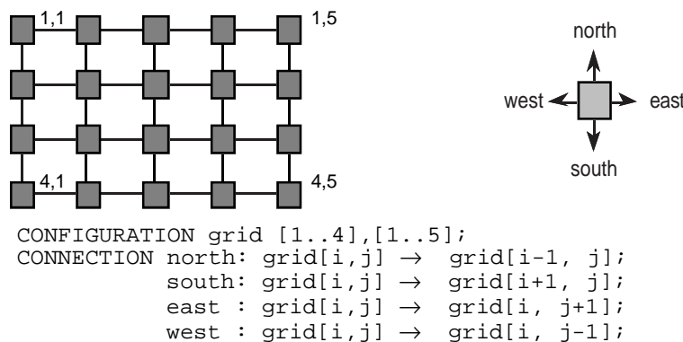
Figure 1.1: Two-dimensional grid topology with representative PE
