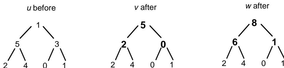
Figure 1.9: Move without and with reduction
