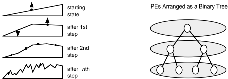
Figure 2.2: Divide-and-conquer implemented with tree topology
