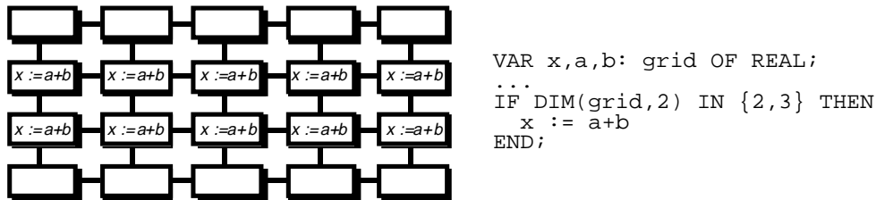
Figure 1.7: Data parallel instruction
