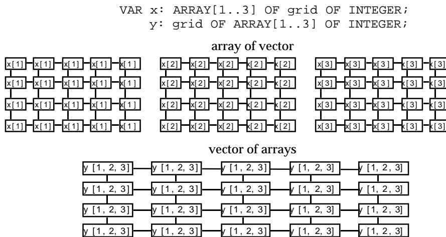
Figure 1.6: Array of vectors and vector of arrays
