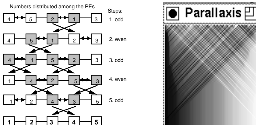
Figure 2.5: Example of odd-even transposition sorting
